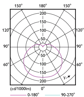
Light Distribution Diagram - TForce Core HB 3.5Klm 40W E27 865
