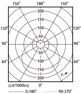
Light Distribution Diagram - TForce Core HB 4.5Klm 50W E27 865
