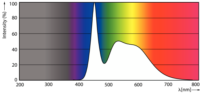
Spectral Power Distribution Colour - TForce Core HB 4.5Klm 50W E27 865
