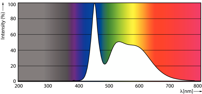
Spectral Power Distribution Colour - TForce Core HB 2Klm 23W E27 865
